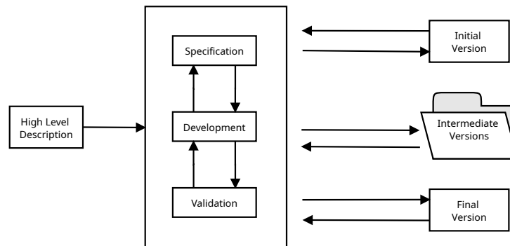
Figure 137: High-level diagram of the evolutionary life cycle model
